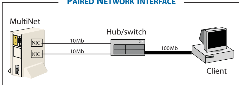
Figure 2 - Dual 10Mb NICs improve throughput by utilizing bandwidth on a 100Mb Ethernet segment downstream from the server segment. The Paired Network Interface combines failover with an ability to use existing network interface cards as well as increase transmission performance from the server.
